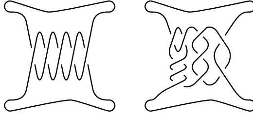
Figure 5: 5_1 and 10_{132}
