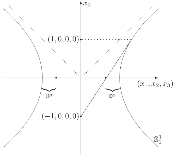
FIGURE 1. The projection p .
