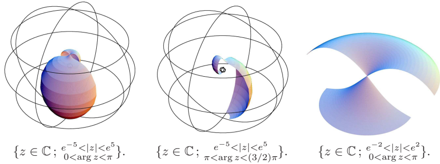
FIGURE 5. Pictures of Example 5.4, where \mu = 0.8 .
