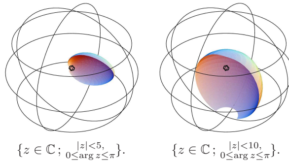
FIGURE 2. Pictures of Example 5.1. The left-hand side is drawn with c_1 = 1.2 , c_2 = 1 and the right-hand side is drawn with c_1 = 0 , c_2 = 1 .
