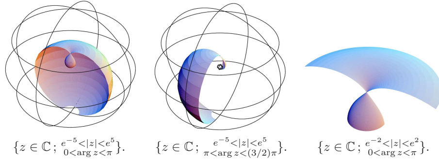
FIGURE 6. Pictures of Example 5.4, where \mu = 1.2 .
