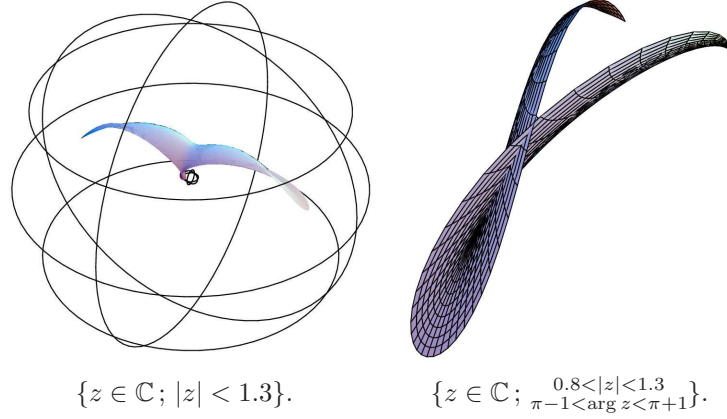
FIGURE 3. Pictures of Example 5.2, where c = 1 .
