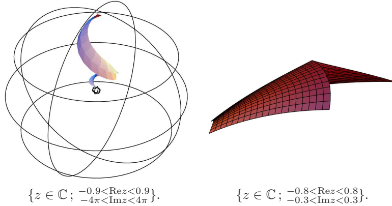
FIGURE 4. Pictures of Example 5.3, where c = 1 .
