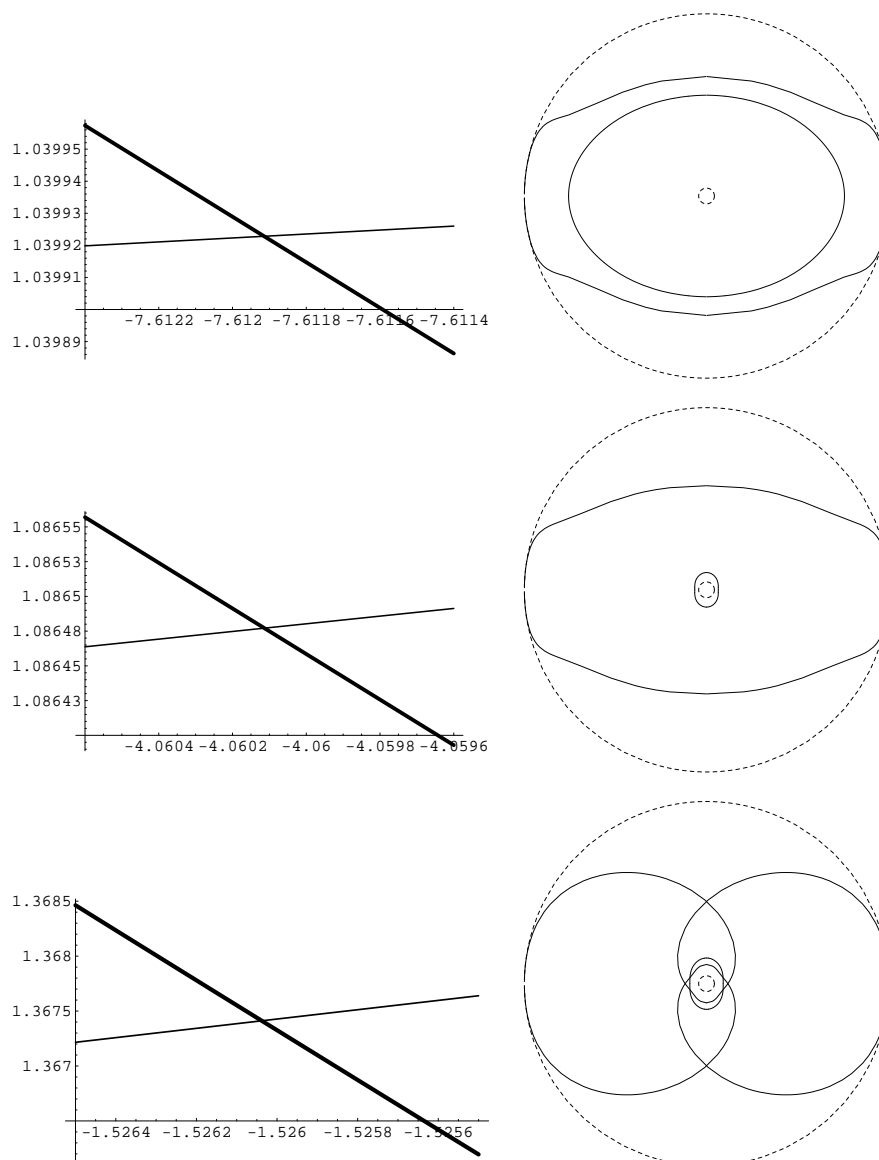
FIGURE 6.4.3. Left: The function f_1 (thin curve) and f_2 (thick curve) when a = 2 . The horizontal axis represents c , and the vertical axis represents f_1 and f_2 . We see that f_1, f_2 > 1 for c \in (-7.6124, -7.6114) in the first row, c \in (-4.0606, -4.0596) in the second row and c \in (-1.5265, -1.5255) in the third row, and f_1 = f_2 at some such value of c in each case, and a = 2 > 1 . Right: Symmetry curves in the CMC 1 face in Example 6.4.8 intersect the plane \{(y_1, y_2, y_3) \in \mathcal{H} \mid y_2 = 0\} , with a = 2 and c = -7.6119 (resp. c = -4.06015 , c = -1.526035 ).
